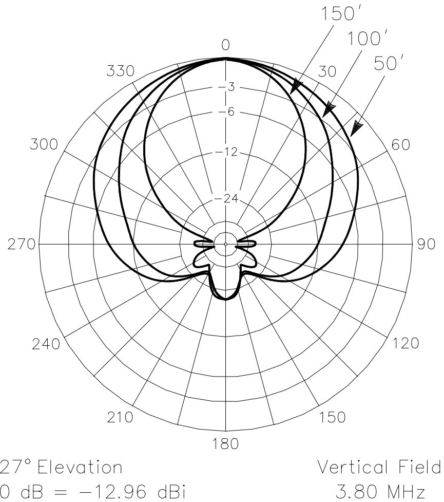
Figure 9—Azimuth patterns of the Figure 8 array for varying degrees of antenna separation.
