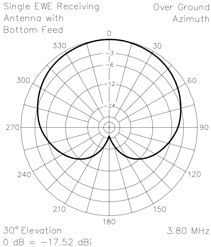
Figure 2A—Azimuth pattern of a single Ewe over average ground.
