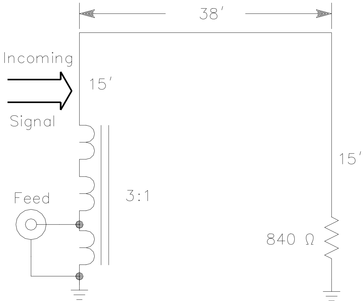
Figure 5—An 160/80-meter Ewe 15 feet high.
