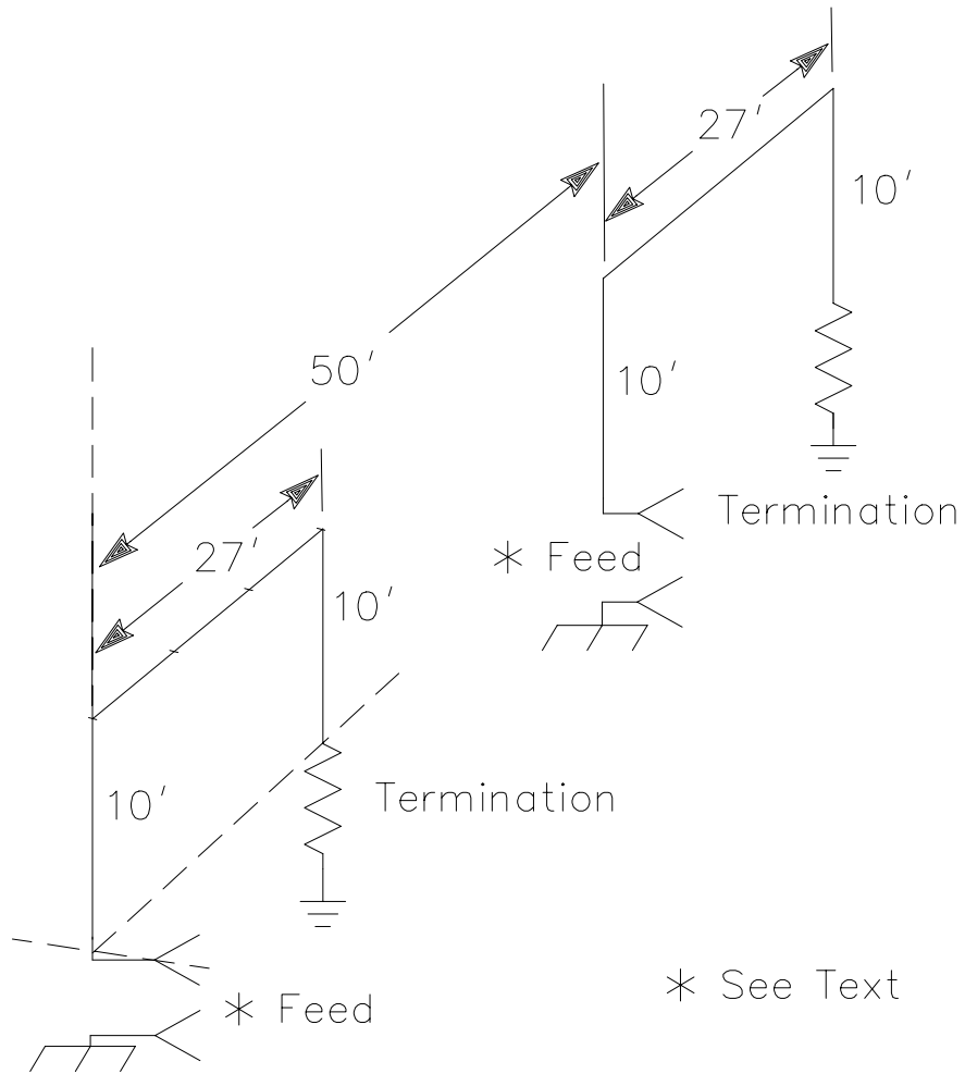
Figure 6—An array of two 10-foot-high Ewes.
