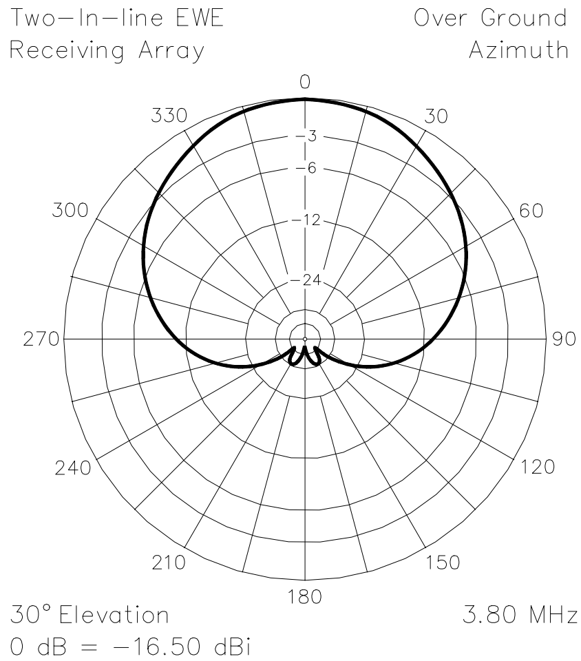
Figure 7A—Azimuth pattern of the dual-Ewe array of Figure 6.
