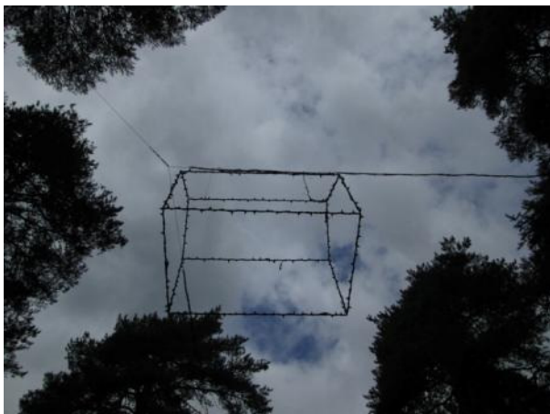
Pentantenna
