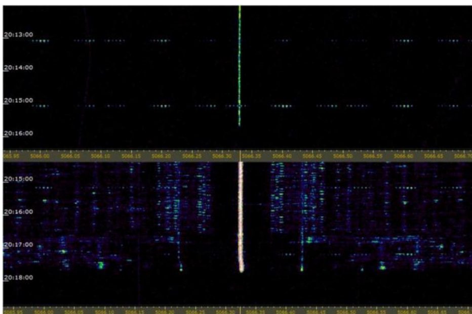
Comparison of 5066,23 R. Candip : top is 2014-12-04 (during R2 radio blackouts and a half hour after 2 solar flares), and bottom is 2014-11-11
